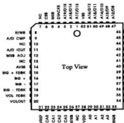
ICS1399V - 52-Lead Plastic Leaded Chip Carrier
