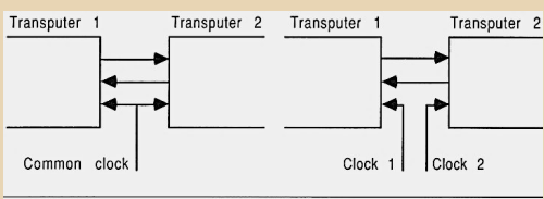
Figure 1.6: Clocking transputers
