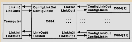
Figure 6.3: Multiple IMS C004 controller
